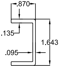
24 REINF. MULLION
