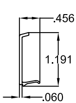
3 GLAZING BEAD
