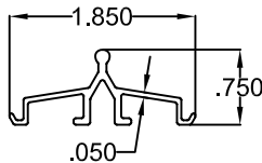
12 ROLLER TRACK
