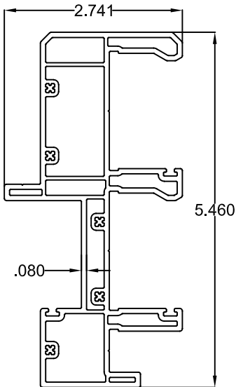
23 MULLION
