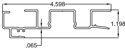
21 HOOKSTRIP
