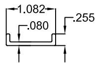
9 ROLLER SUPPORT
